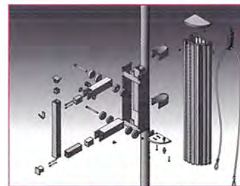
Exploded drawing
